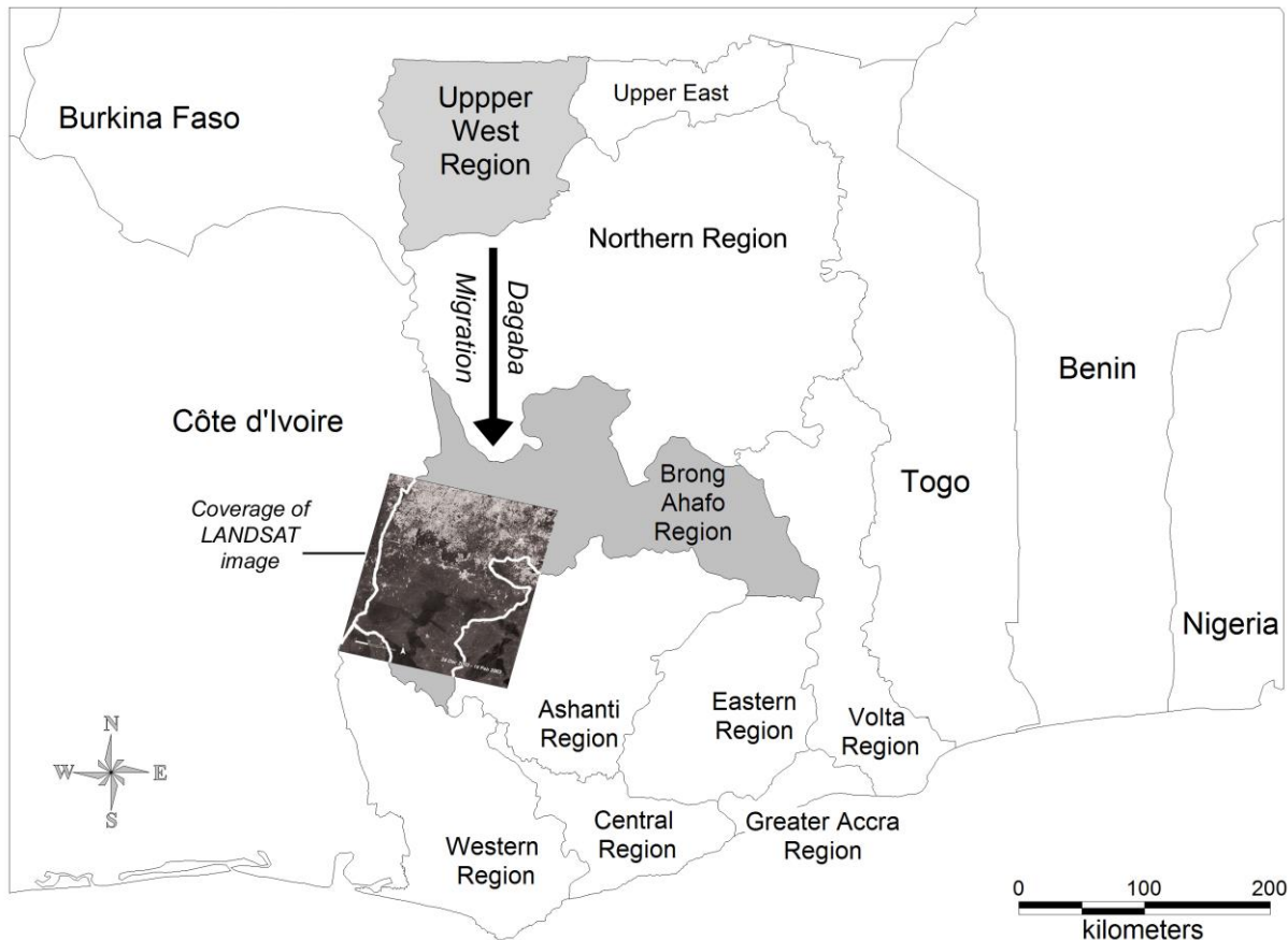
Figure 2: Ghana, Dagaba migration, and coverage of the LANDSAT image
