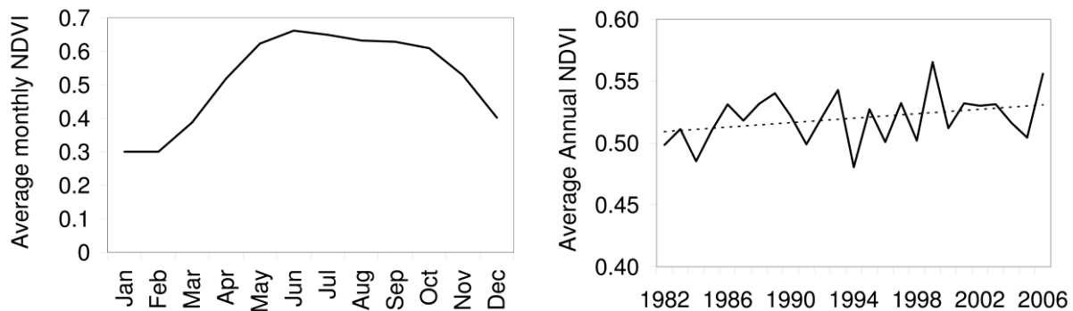
Figure 4: Average monthly NDVI and NDVI trend in the Wenchi District (1982-2006) 13
